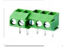
PCB Terminal block 3.50mm & 3.96mm Pitch Right Angle KLS2-350R-3.50 & 3.96
