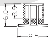
Dimension
