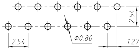
Recommended P.C.B Layout(Top Side) (PCB BOARD TOLERANCE±0.05)
