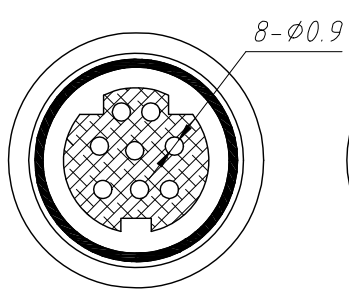
8 Pin
