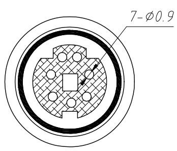
7 Pin
