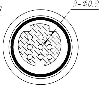
9 Pin
