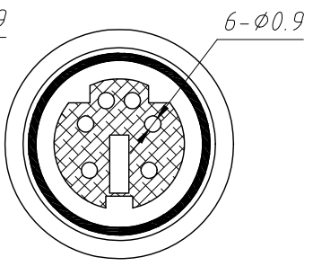
6 Pin
