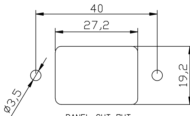
PANEL CUT-OUT
