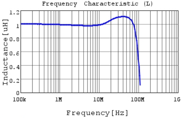
LQM21PN1R0MC0 L
