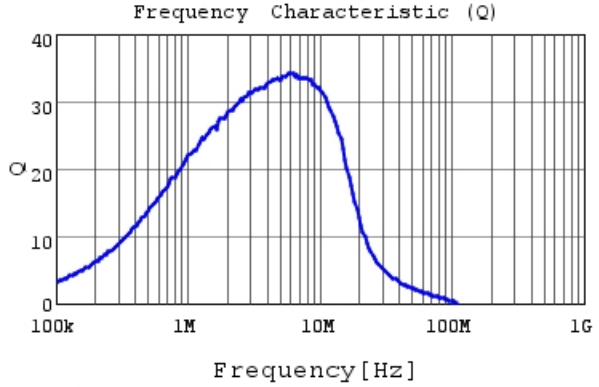
LQM21PN1R0MC0 Q
