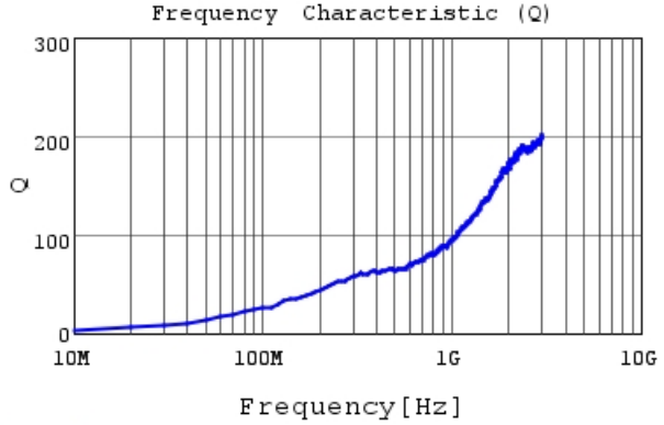
LQP15MN1N0W02 Q
