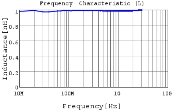
LQP15MN1N0W02 L
