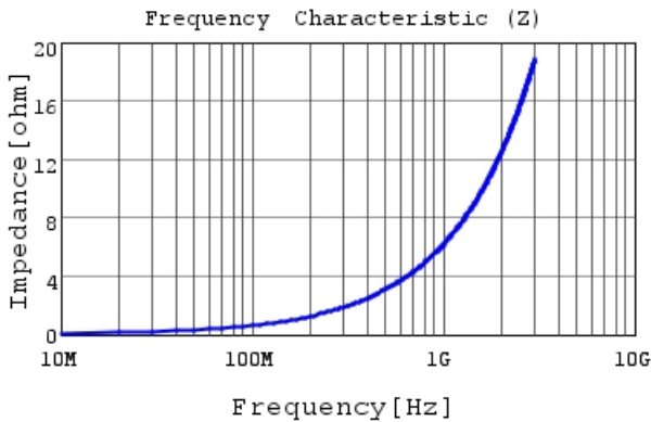
LQP15MN1N0W02 |Z|
