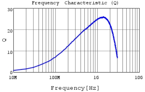
LQP15MN22NG02 Q
