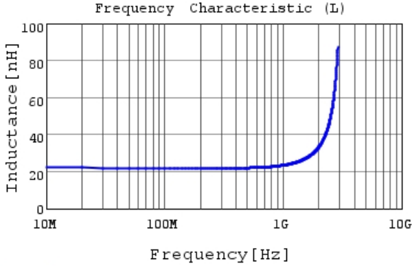
LQP15MN22NG02 L
