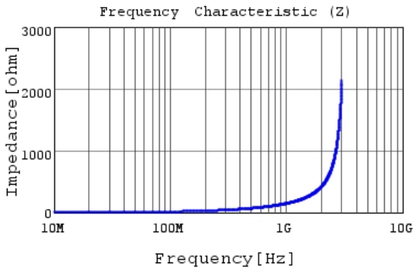
LQP15MN22NG02 |Z|
