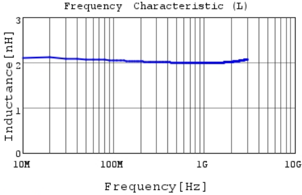
LQP15MN2N0B02 L
