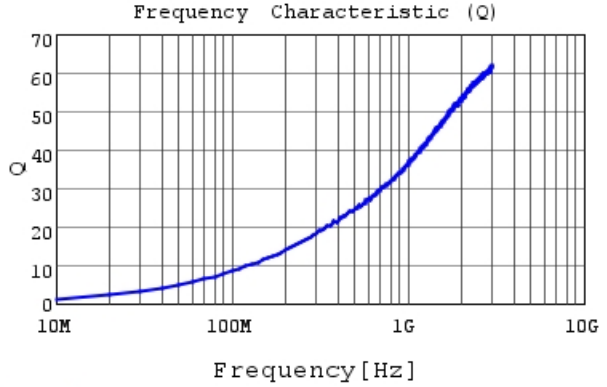
LQP15MN2N0B02 Q
