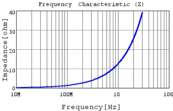
LQP15MN2N0B02 |Z|
