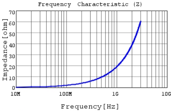
LQP15MN3N0W02 |Z|
