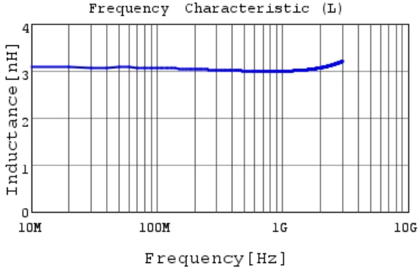
LQP15MN3N0W02 L
