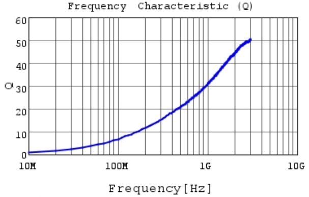
LQP15MN3N0W02 Q
