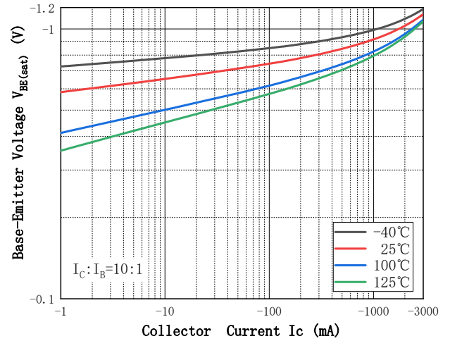
Fig.4 - Base-Emittor Voltage
