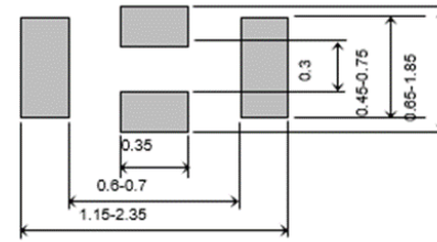
NFM15HC
