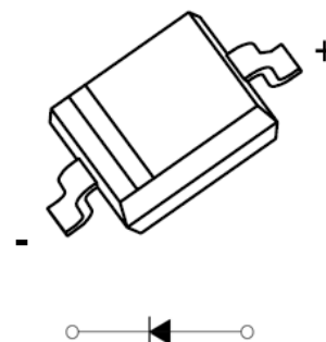
SOD-323
