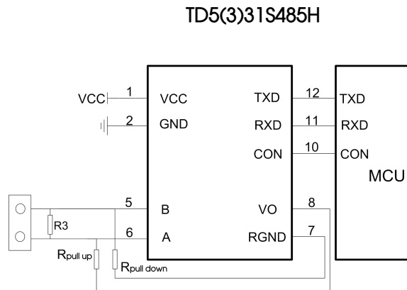
Fig. 1: Typical application
