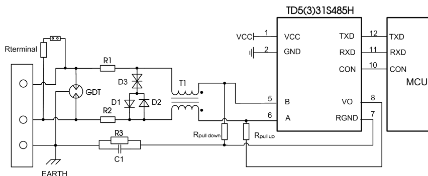
Fig. 2: Port protection circuit for harsh environments
