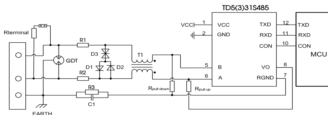
Fig. 2: Port protection circuit for harsh environments
