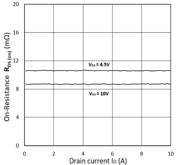
Figure 6. R_{DS(on)} vs. V_{GS}
