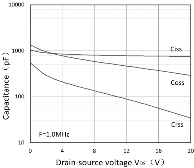
Figure 7. Capacitance Characteristics
