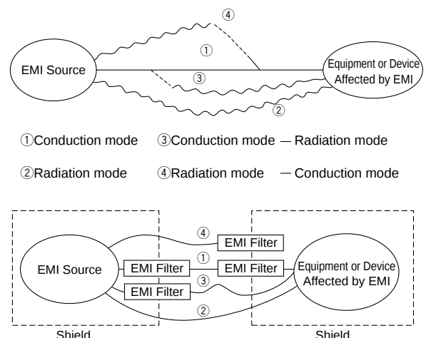
EMI Propagation Mode and Model of Noise Filter Suppression
